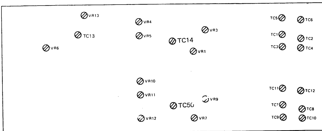
Fig. 13 VERTICAL AMPLIFIER UNIT 290-1016-34
