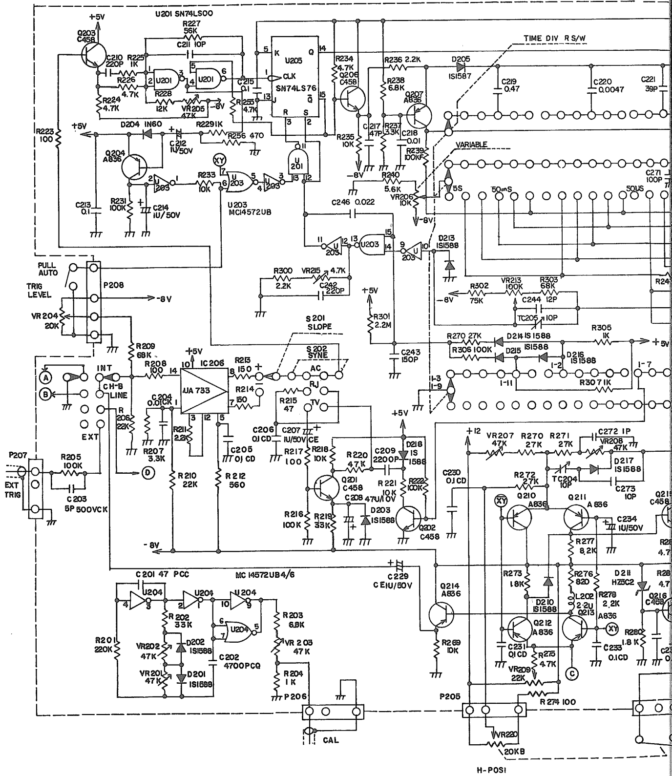
7-2-(1) HORIZONTAL/TIME BASE CIRCUIT DIAG
